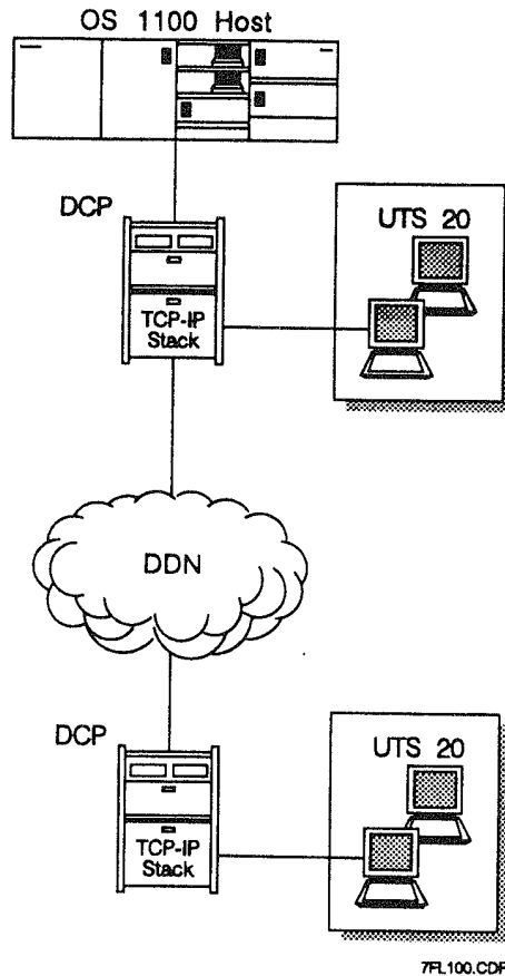
Figure A-5. DCP-to-DCP Trunk over the DDN
