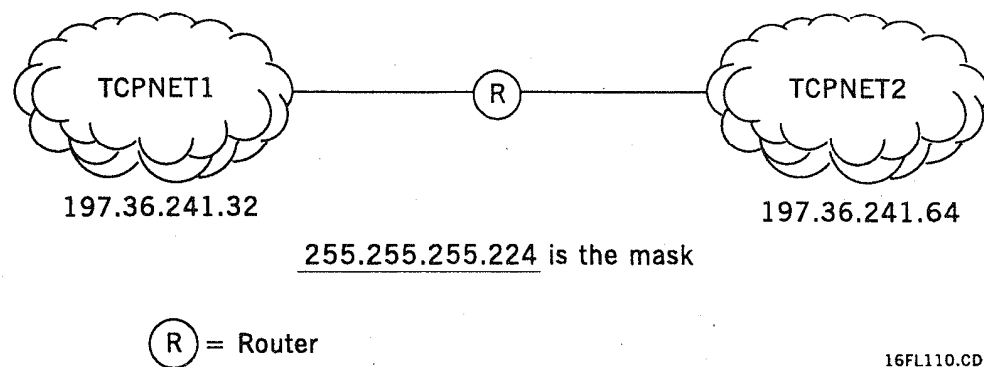
Figure 2-1. Subnetwork Topology
